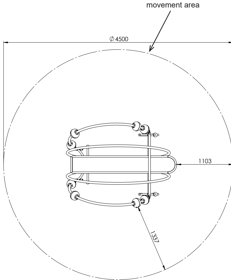
Diagram 3: Top view
